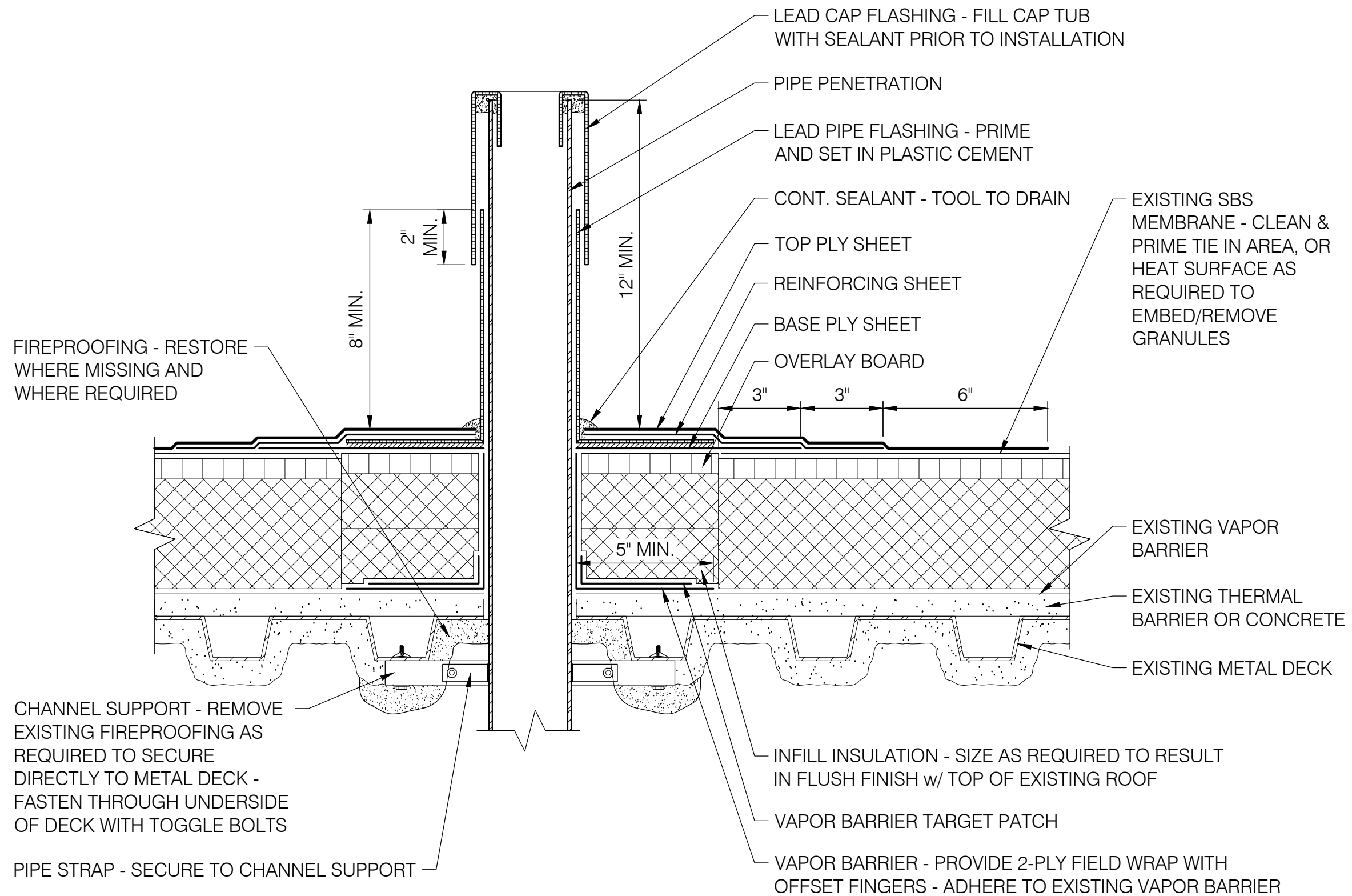
0710 SBS FLASHING - PLUMBING VENT FLASHING SCALE: 3" = 1'-0"
