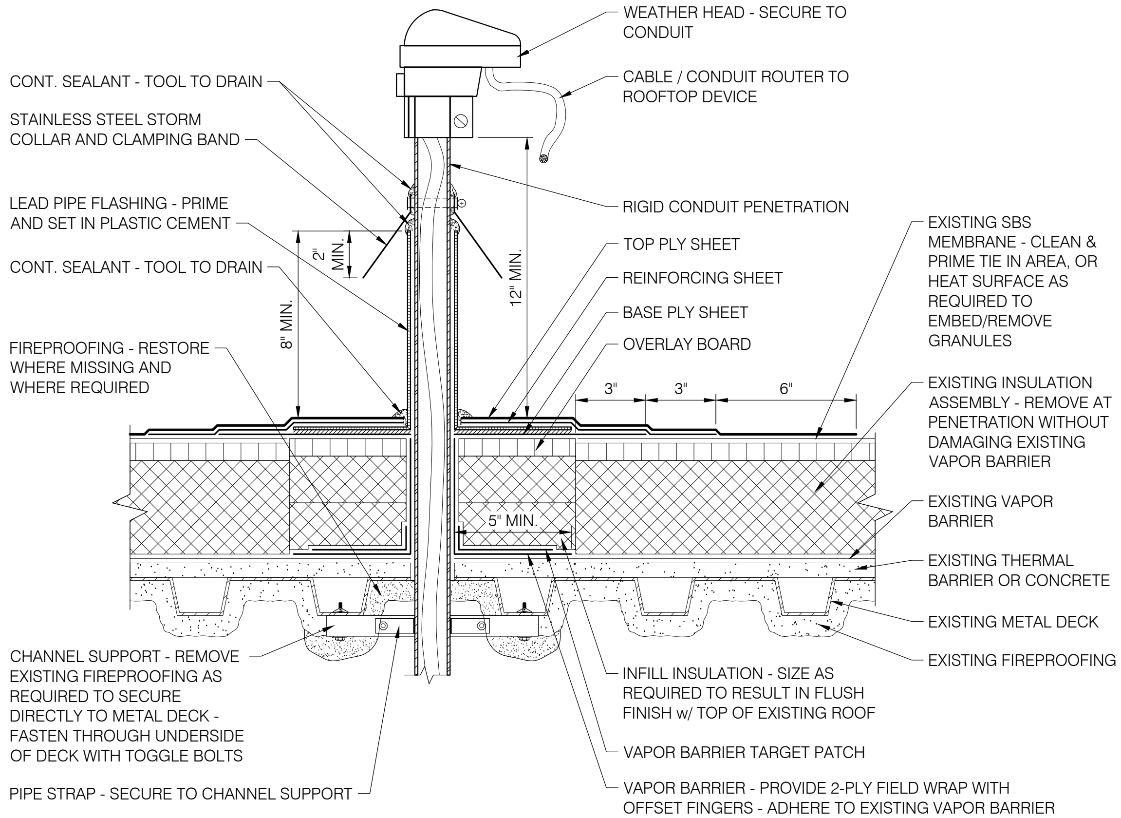
0712 SBS FLASHING - WEATHERHEAD MAST SCALE: 3" = 1'-0"
