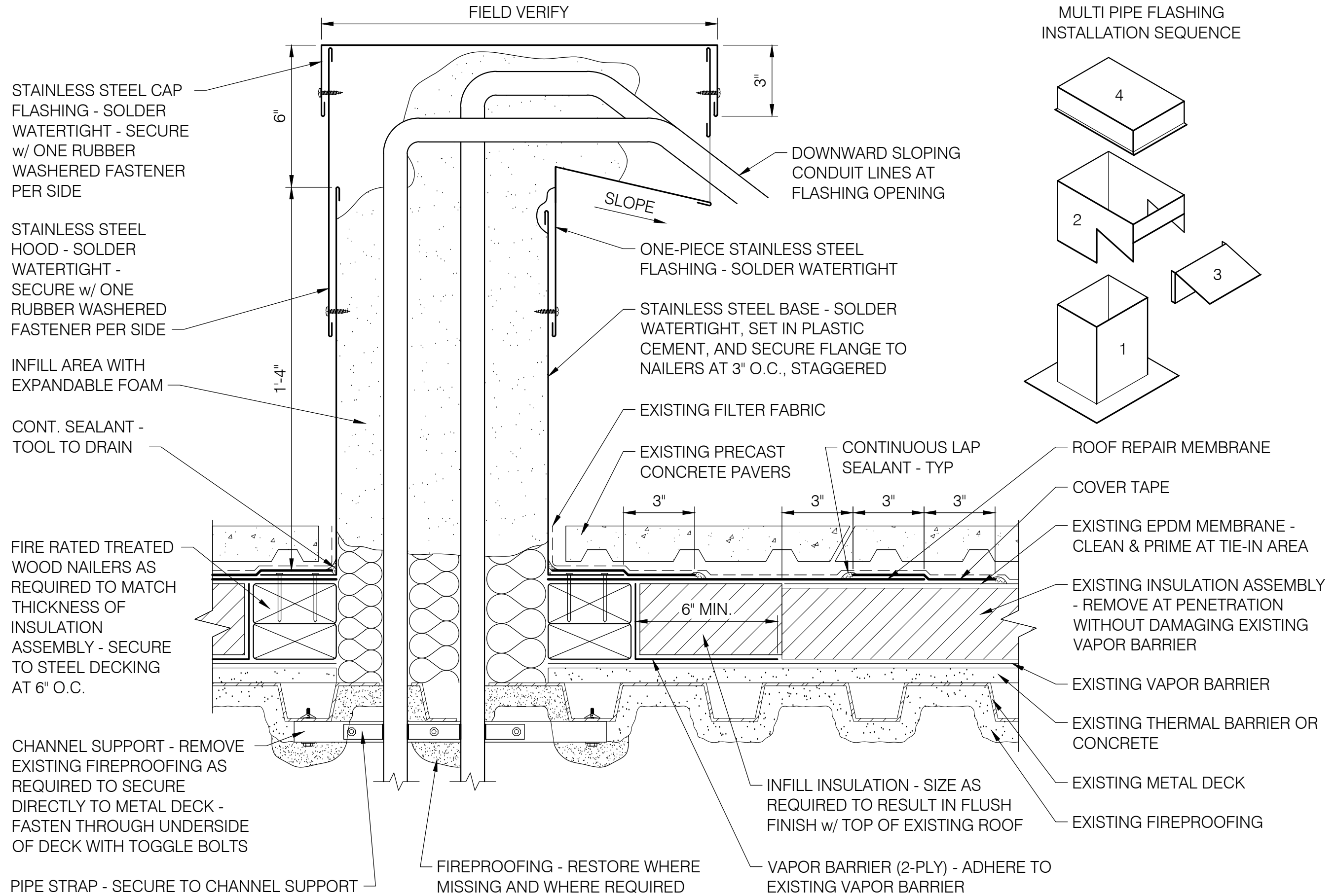
0729 EPDM FLASHING - MULTIPLE PIPE PENETRATION SCALE: 3" = 1'-0"
