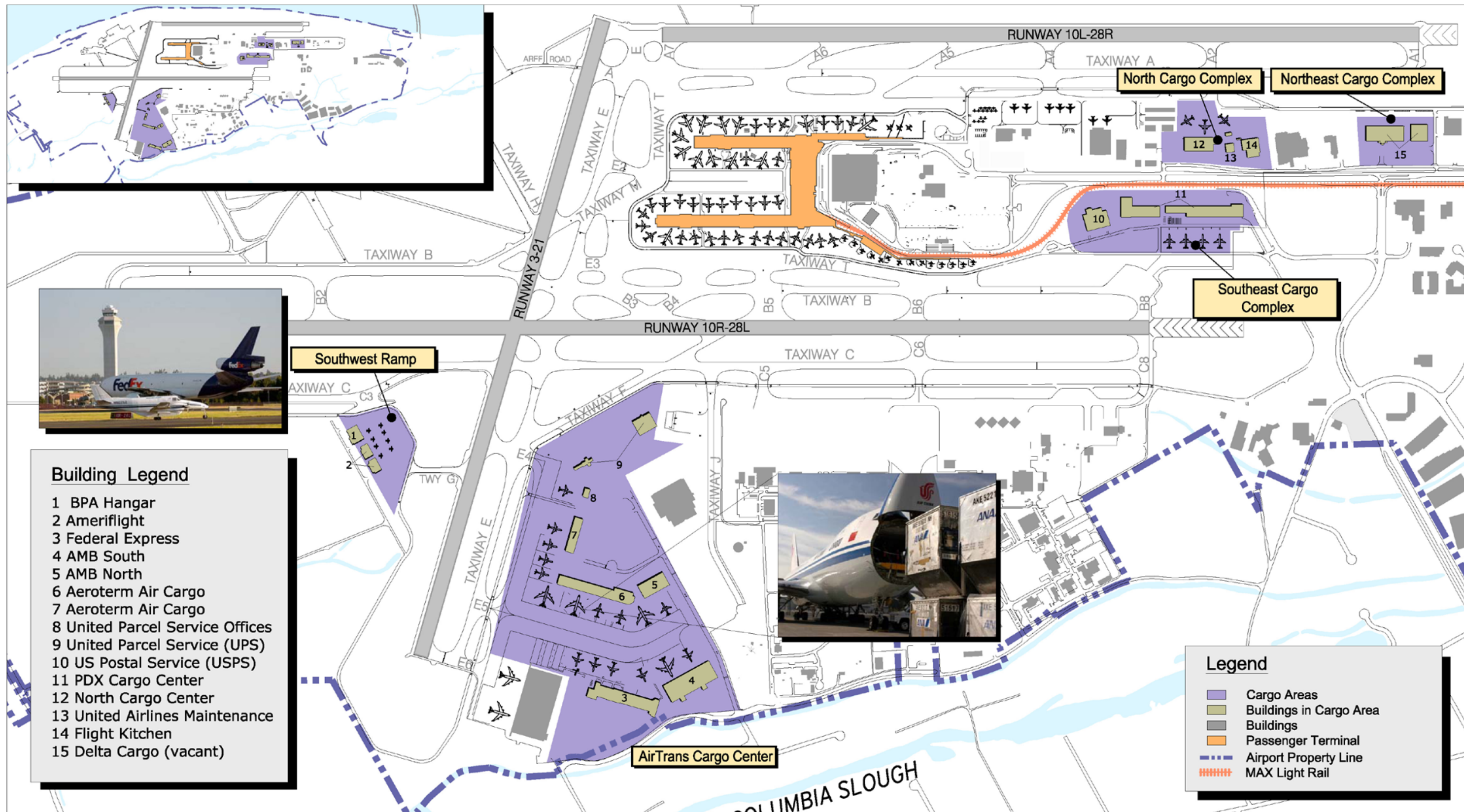
Figure 5-41 Cargo Areas Master Plan Update Portland International Airport
