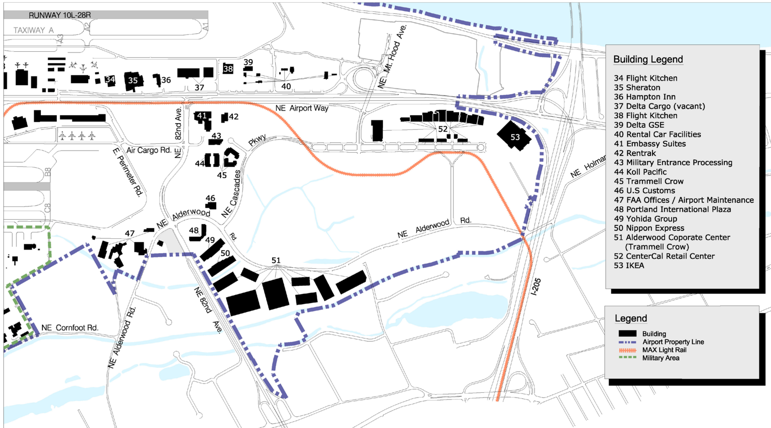
Figure 5-4 Airport Facilities - East Master Plan Update Portland International Airport
