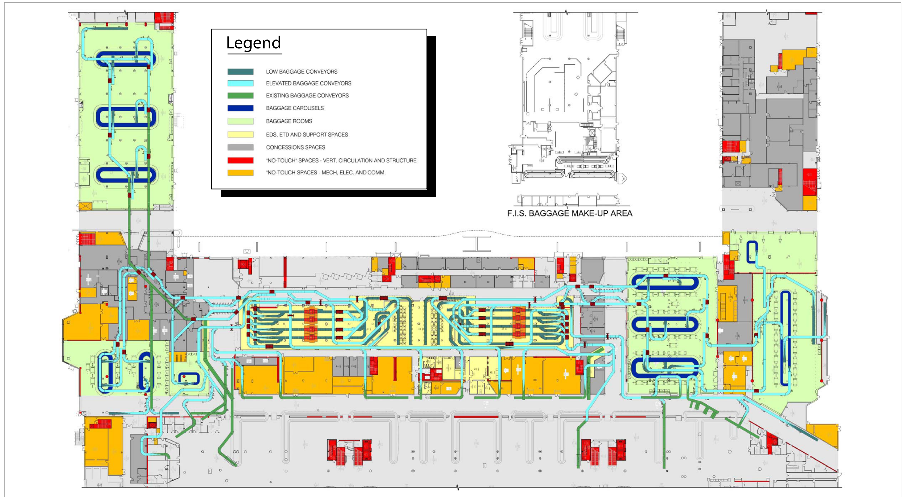
Figure 5-23 In-Line Baggage Screening System (First Floor)
