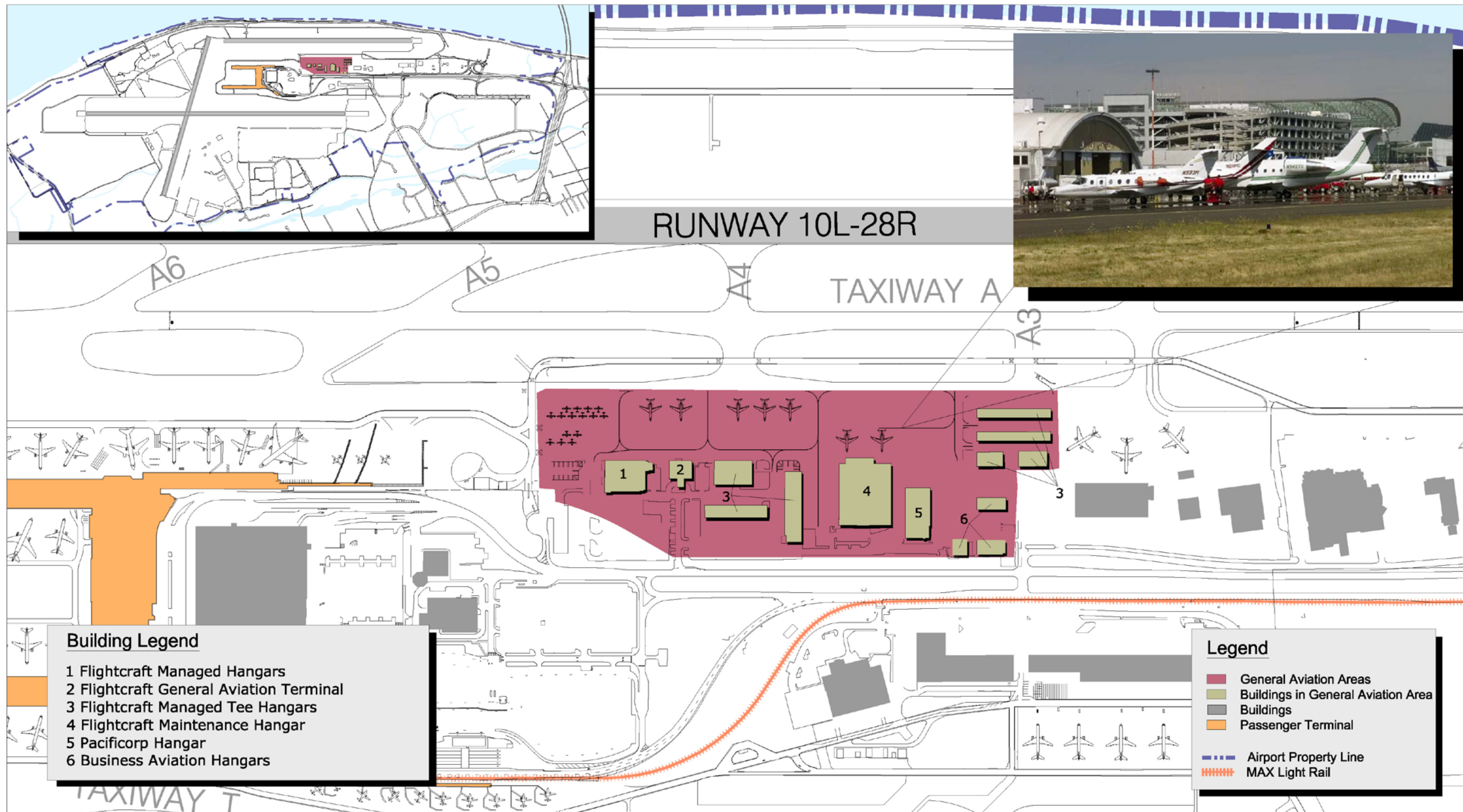
Figure 5-42 General Aviation Area Master Plan Update Portland International Airport
