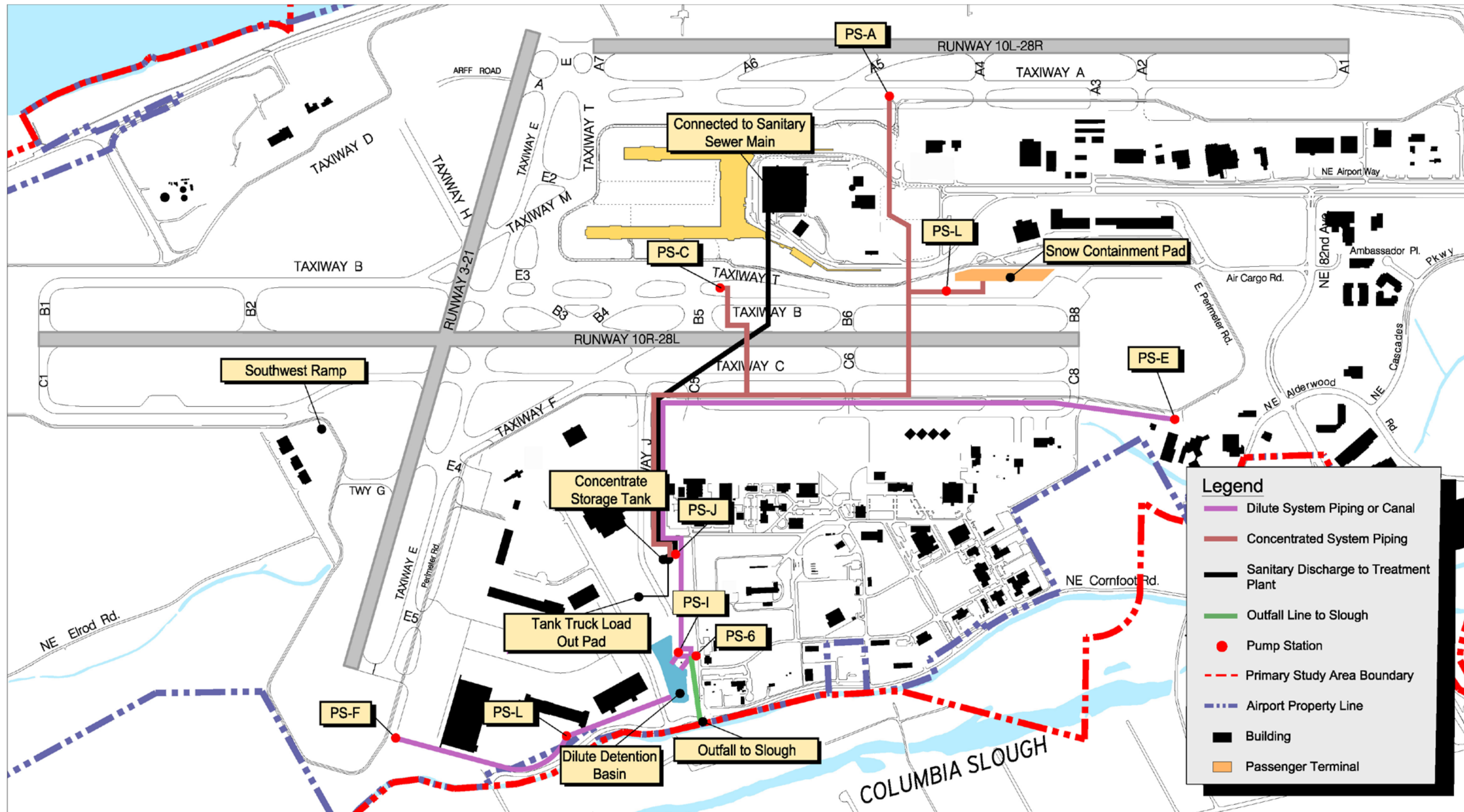
Figure 5-45 Deicing System Basic Diagram Master Plan Update Portland International Airport
