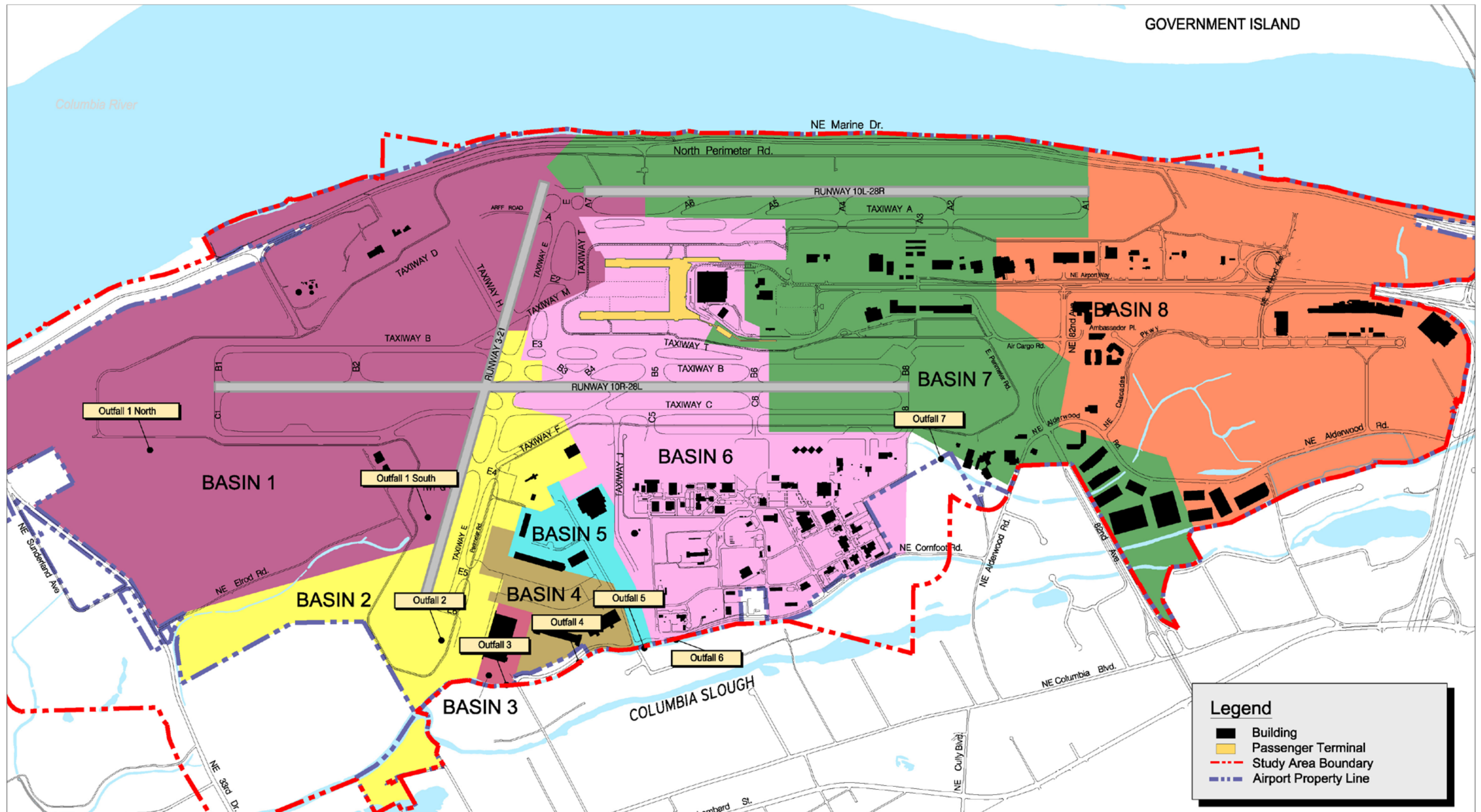
Figure 5-47 Stormwater Drainage Basins Master Plan Update Portland International Airport September 2008
