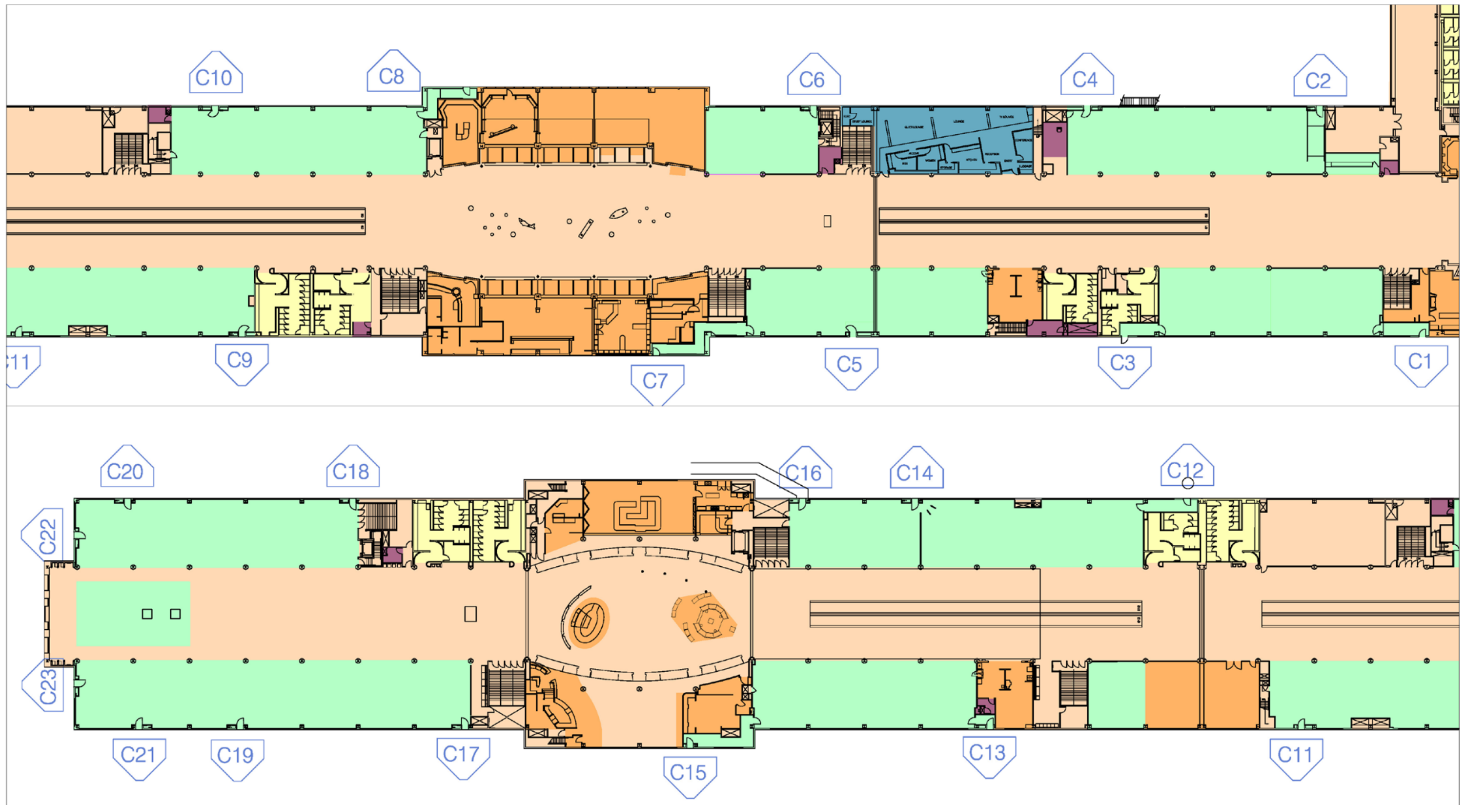
Figure 5-17 Concourse C: Enplaning Level (Second Floor)
