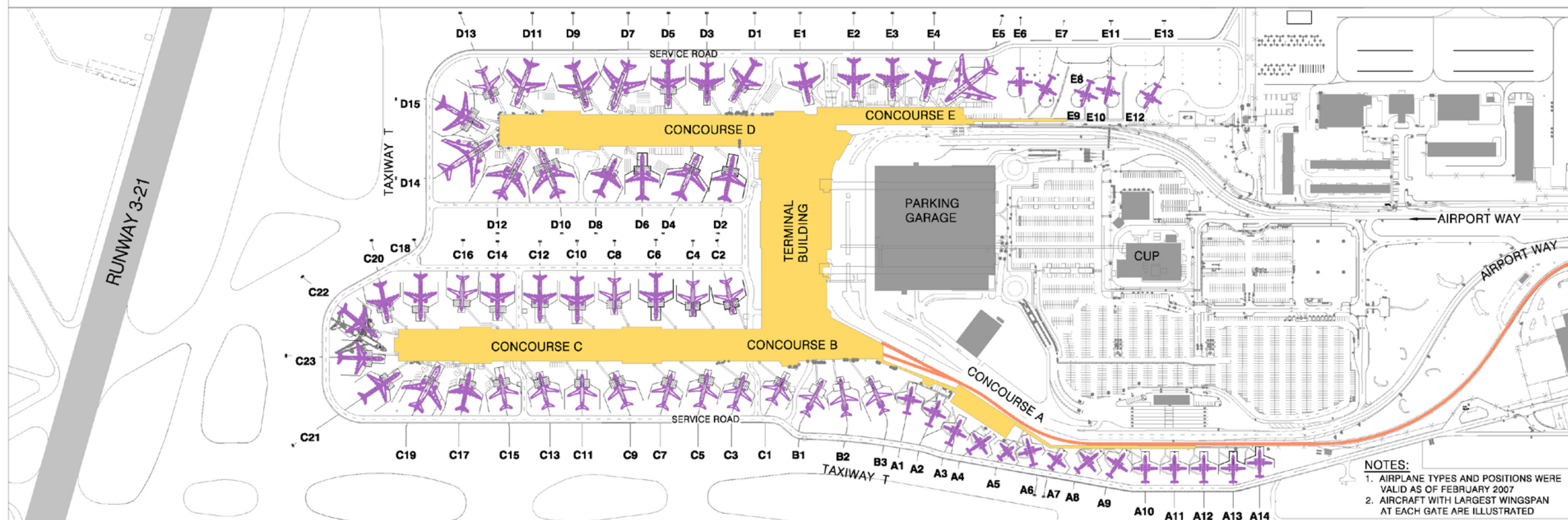
Figure 5-7 Gate Locations and Aircraft Parking Master Plan Update Portland International Airport September 2008
